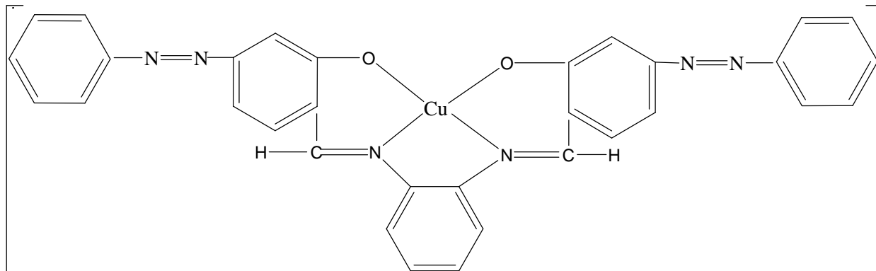
Figure.1 proposed molecular structure of the copper (II) Schiff base complex.
