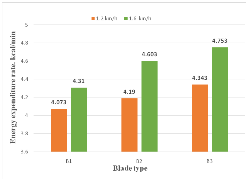
Fig.5 Effect of forward speed of weeder on energy expenditure rate of operator
