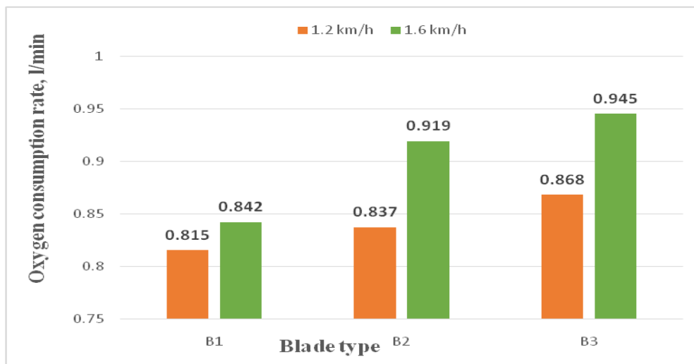
Fig.4 Effect of forward speed of weeder on oxygen consumption rate of operator
