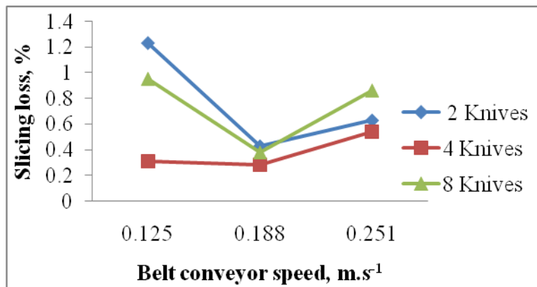
Fig.4 Effect of belt conveyor speed and number of knives on slicing loss (%)
