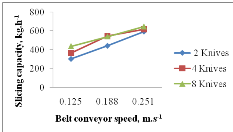
Fig.2 Effect of belt conveyor speed and number of knives on slicing capacity (kg.h)
